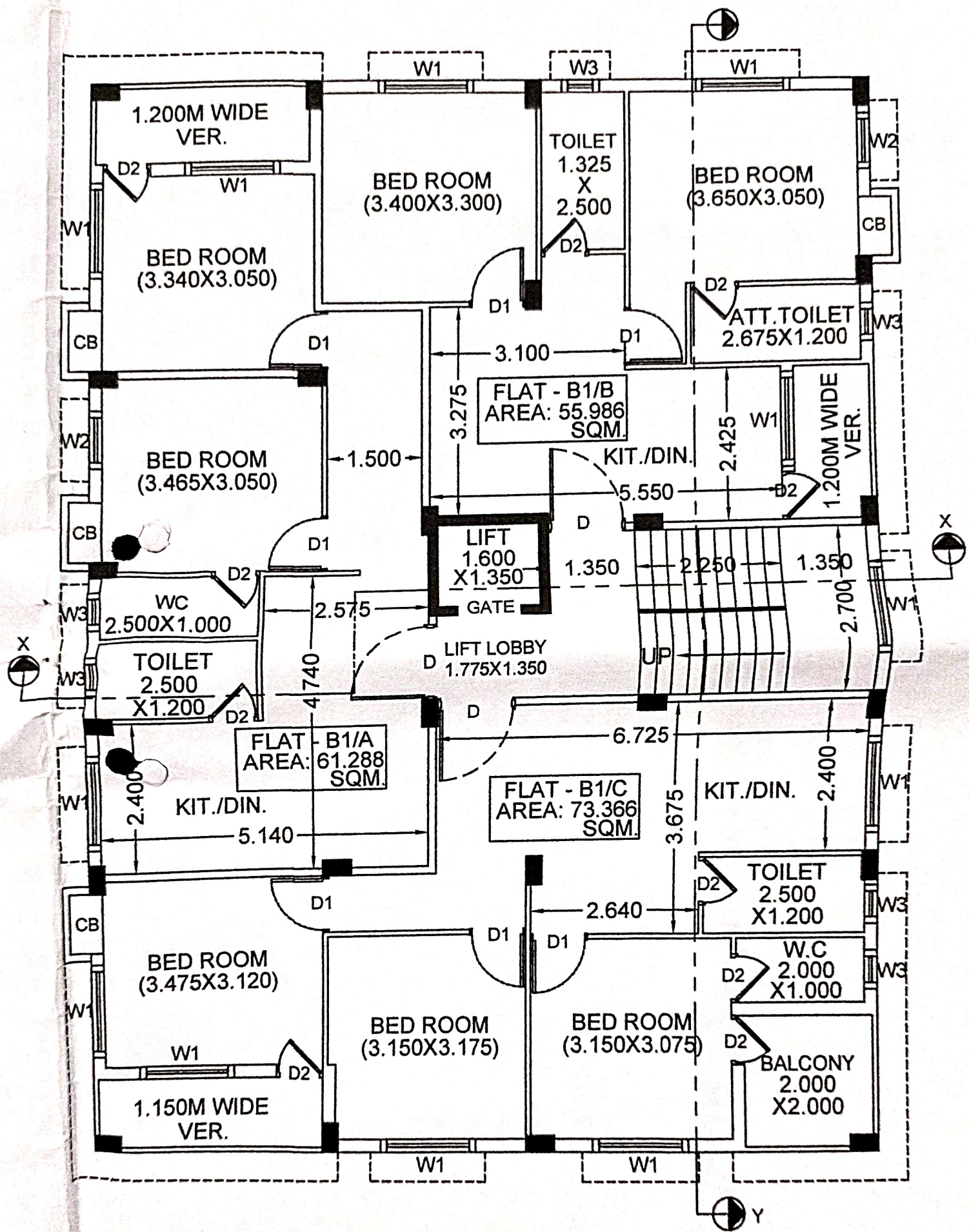
PROPOSED TYPICAL FLOOR PLAN OF BLOCK-1 (SCALE - 1:100)
